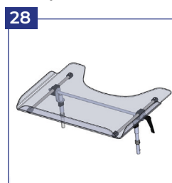
28 Therapy tray, height adjustable
